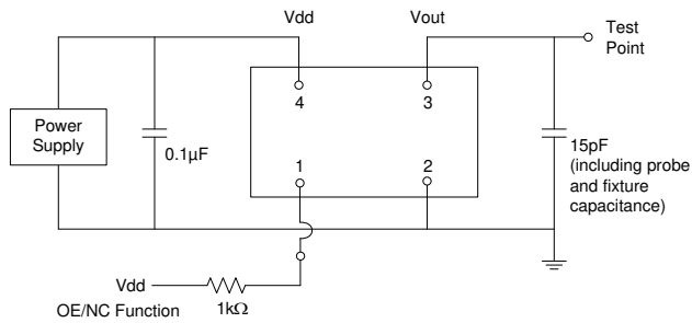
Figure 2. Test Circuit
