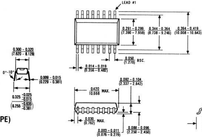
16 Lead Small Outline, Wide (WE) \theta_{JA} = 105^{\circ}\text{C/W} \theta_{JC} = 60^{\circ}\text{C/W}
