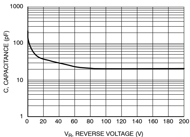
Figure 2. Typical Capacitance
