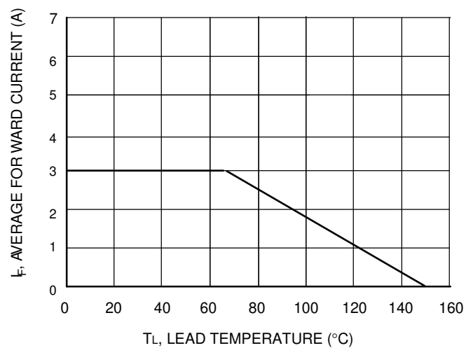
Figure 4. Derating Curve
