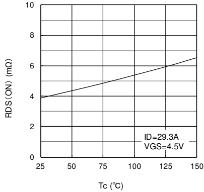
RDS(ON)-Tc characteristics (typical) ID=29.3A, VGS=4.5V
