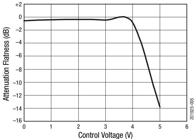
Figure 5. Attenuation Flatness vs Control Voltage (f = 2.1 to 3.1 GHz)
