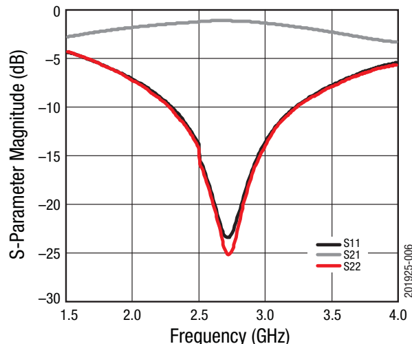
Figure 6. S-Parameter Magnitude vs Frequency
