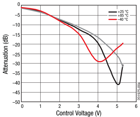
Figure 4. Attenuation vs Control Voltage Over Temperature (f = 2.6 GHz)
