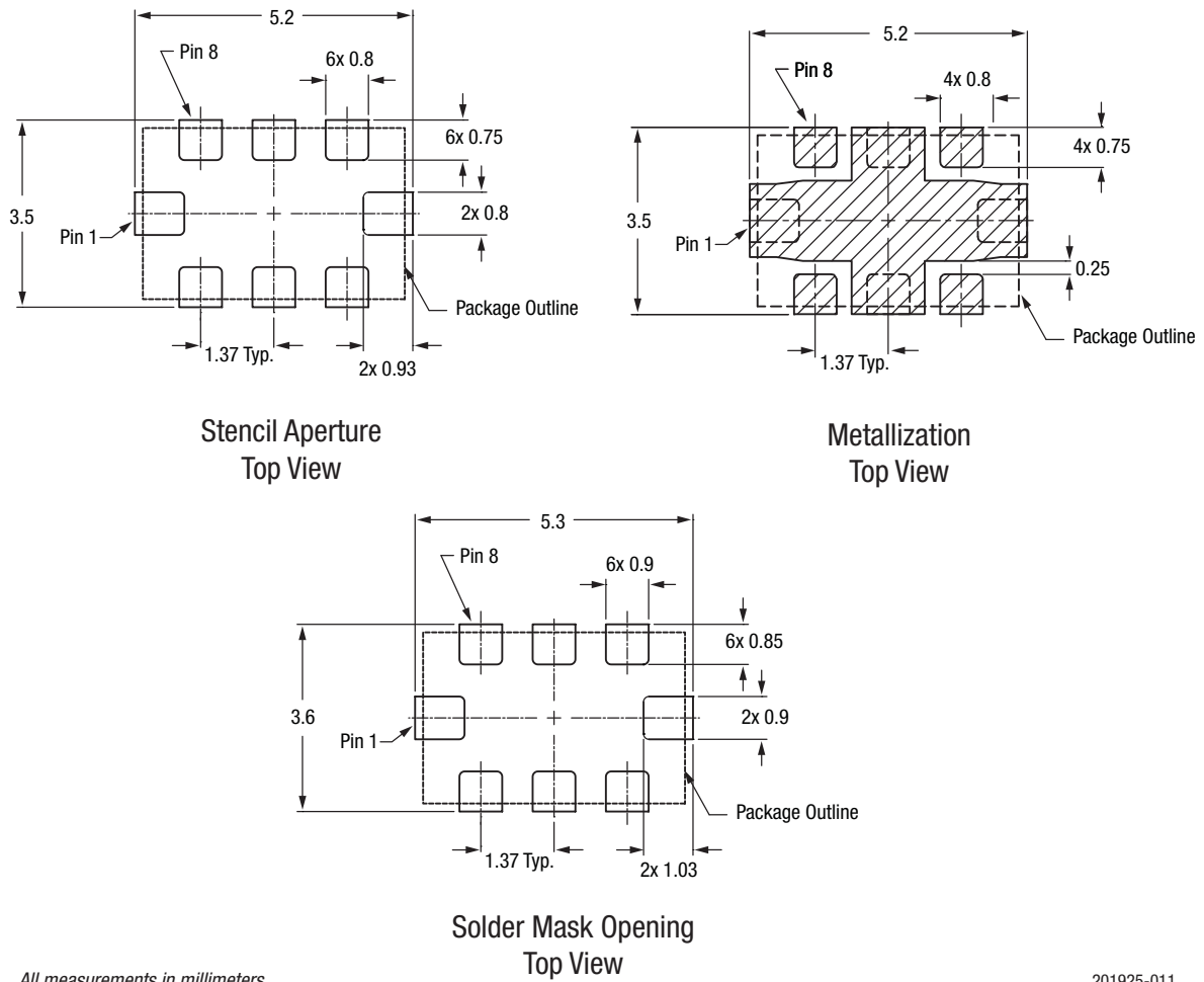
Figure 11. SKY12233-11 PCB Layout Footprint
