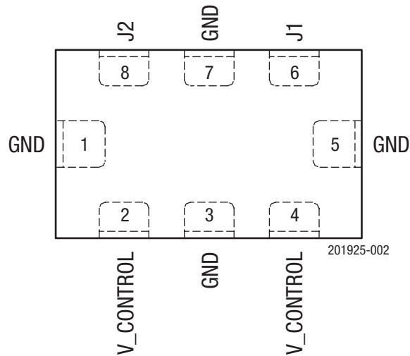
Figure 2. SKY12233-11 Pinout (Top View)
