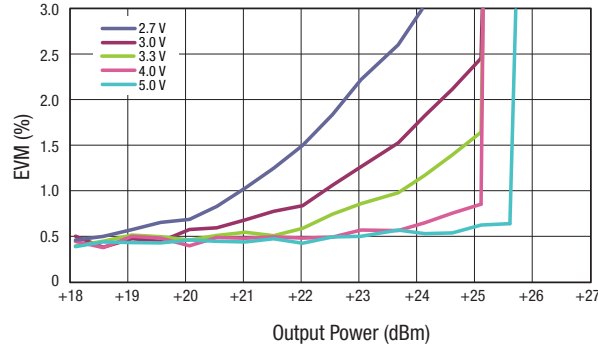
Figure 9. 802.11a EVM vs Output Power, 5.2-5.8 GHz, 54 Mbps
