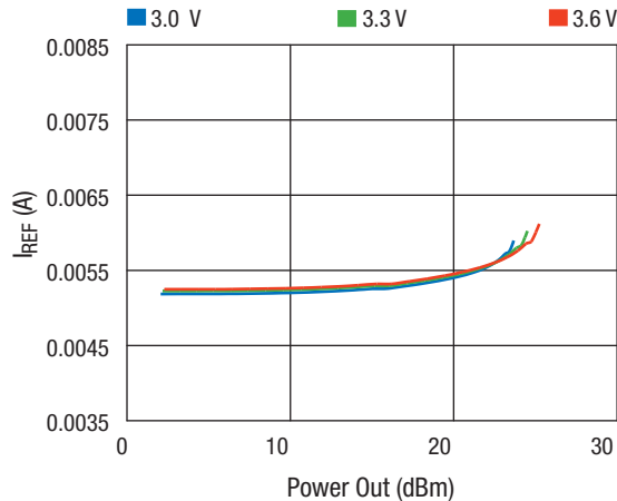
Figure 30. Iref vs Power Out Across Vcc
