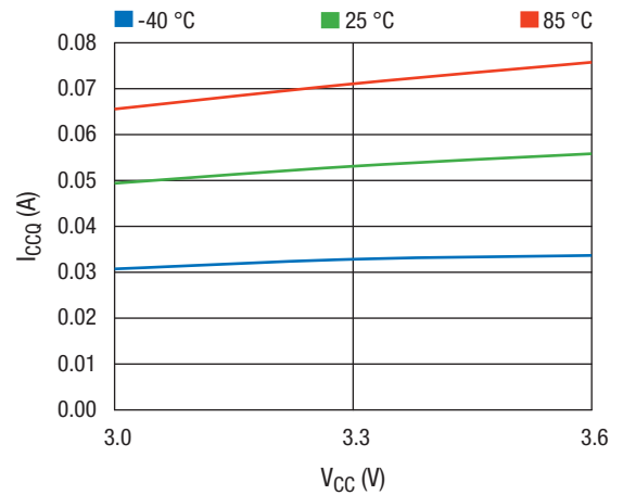
Figure 14. Iccq vs. VCC Across Temperature
