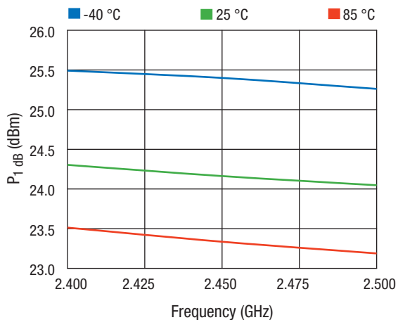
Figure 26. Output P1dB vs Frequency Across Temperature
