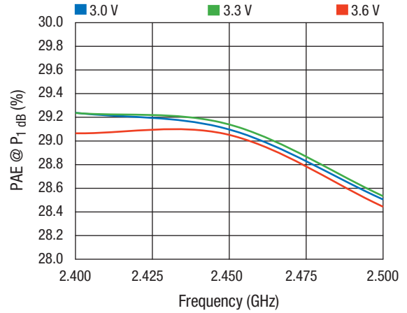
Figure 10. PAE @ P1dB vs Frequency Across VCC
