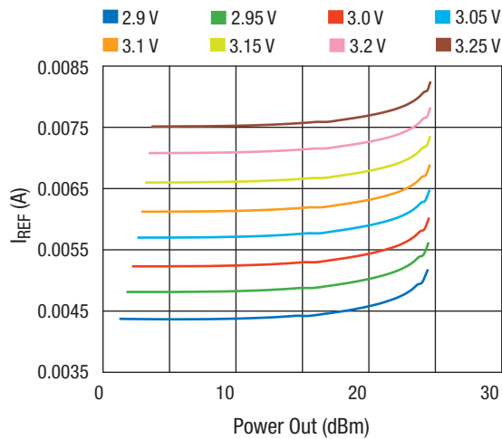
Figure 32. Iref vs Power Out Across Vreg
