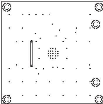
Layer 3: Ground
