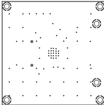
Layer 2: Ground
