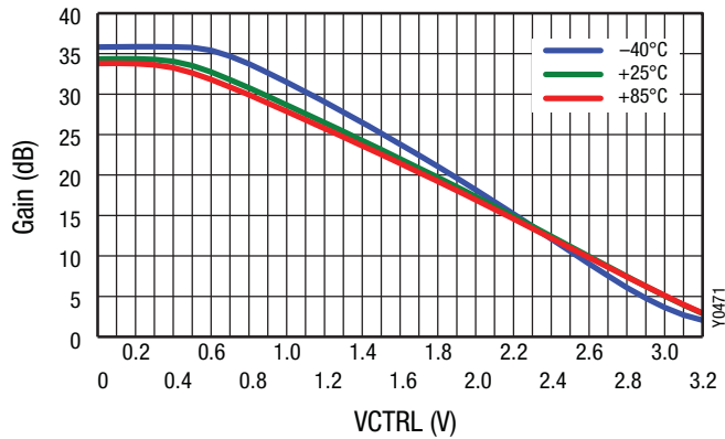
Figure 11. Gain vs VCTRL over Temperature
