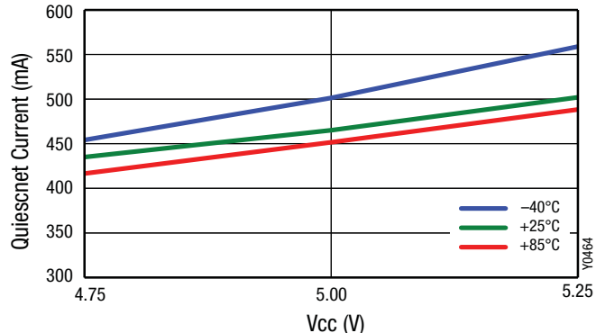
Figure 4. Quiescent Current vs Voltage over Temperature
