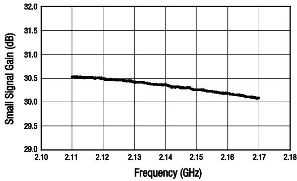
Figure 3. Small Signal Gain vs Frequency
