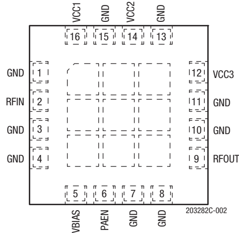
Figure 2. SKY66292-11 Pinout (Top View)
