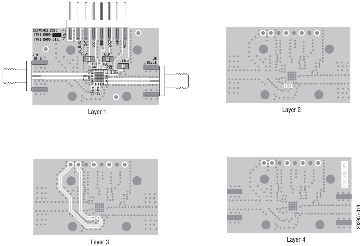
Figure 19. Board Layer Detail
