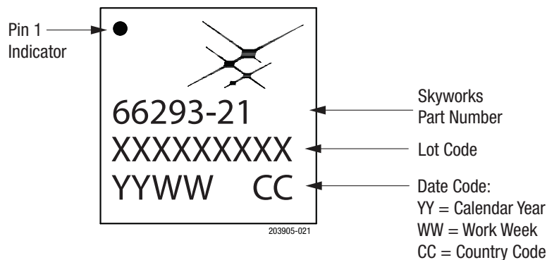
Figure 21. Typical Part Marking for the SKY66293-21
