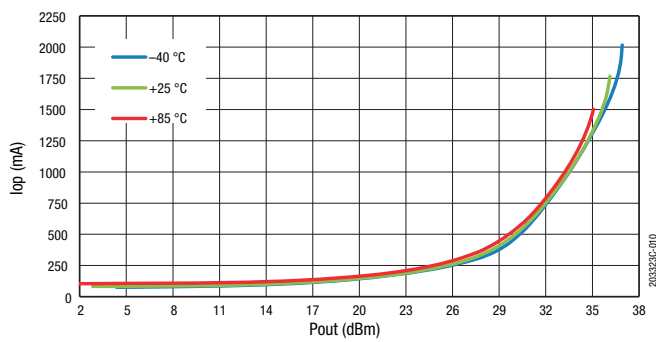
Figure 10. Operating Current vs Pout Across Temperature (CW)
