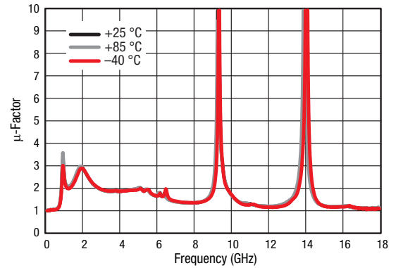
Figure 18. Stability Factor ( \mu ) vs Frequency Over Temperature @ 5 V
