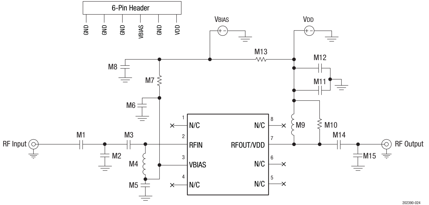
Figure 24. SKY67151-396LF Evaluation Board Schematic (700 to 3800 MHz)
