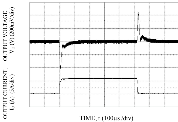
Transient Response to Dynamic Load Change from 0% to 50% to 0%. V_o=3.3V
