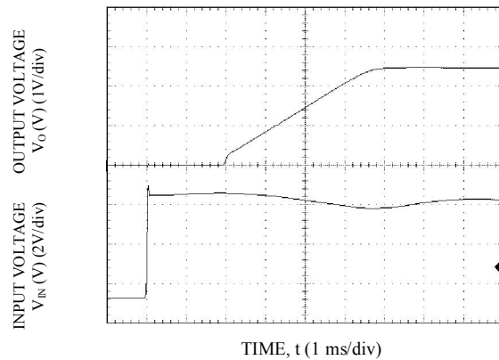
Start-up Using Input Voltage ( V_{IN} = 5V , I_o = I_{o,max} ), V_o=2.5V
