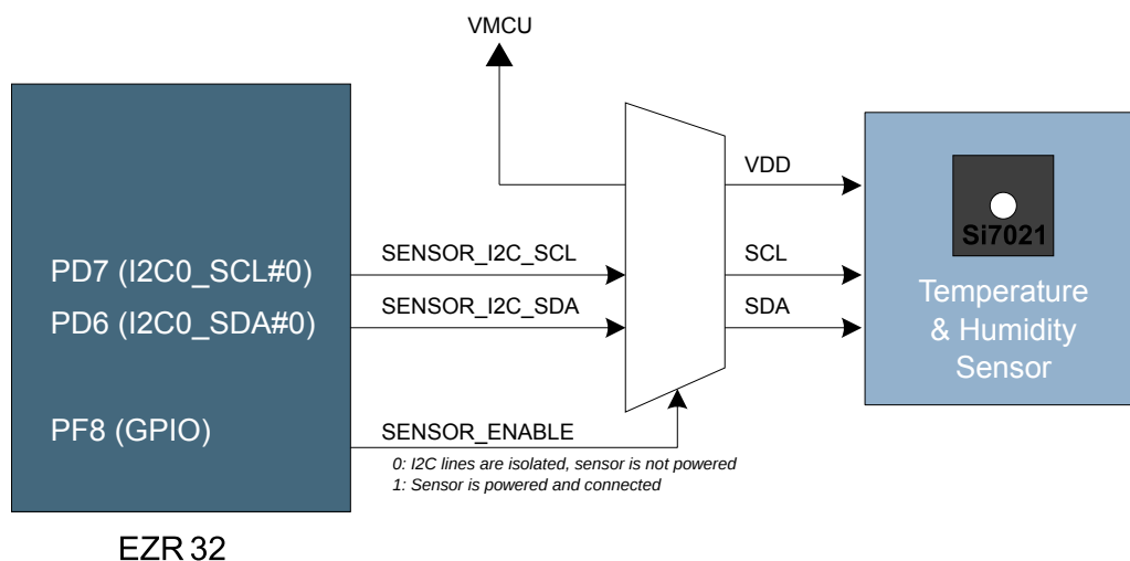
Figure 5.4. Si7021 Relative Humidity and Temperature Sensor
