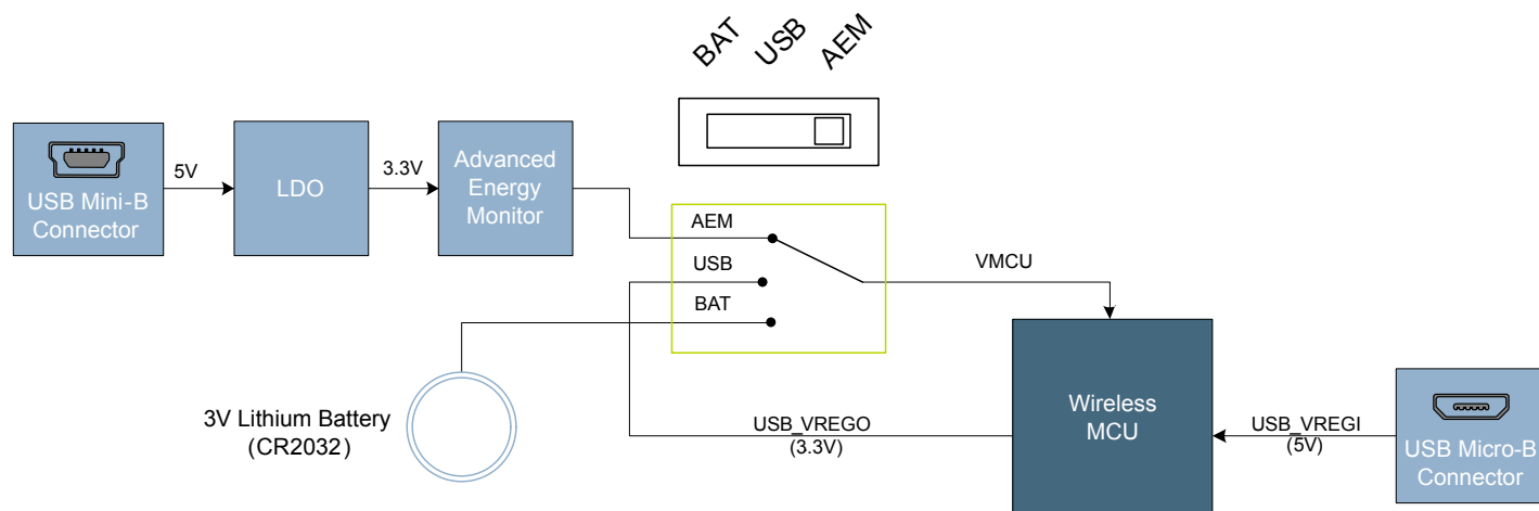
Figure 4.1. WSTK6222 Power Switch
