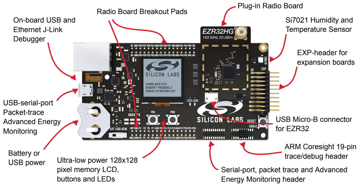
Figure 2.1. SLWSTK6244A Hardware Layout
