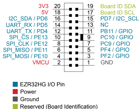
Figure 4.3. Expansion Header
