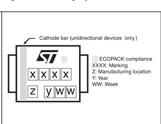
Figure 18. Marking layout (1)
