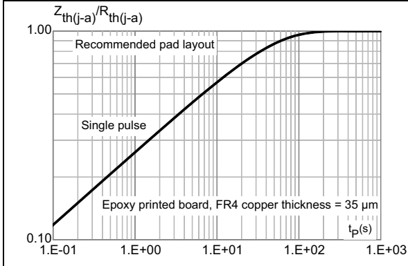
Figure 9. Relative variation of thermal impedance versus pulse duration
