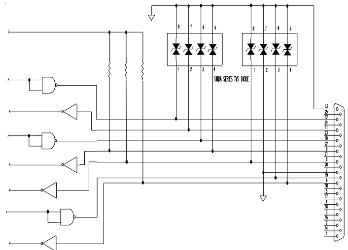
Typical Connection
