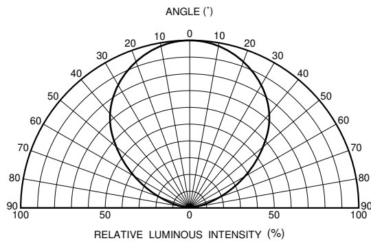
Fig.1 Directional pattern
