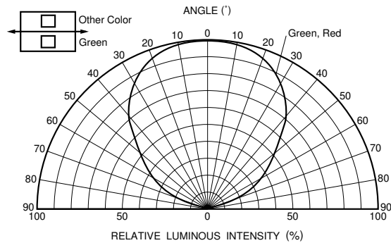
Fig. 2 Directional pattern (2)
