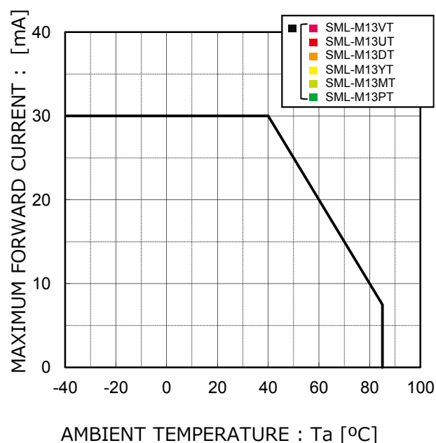
Fig.4 Derating
