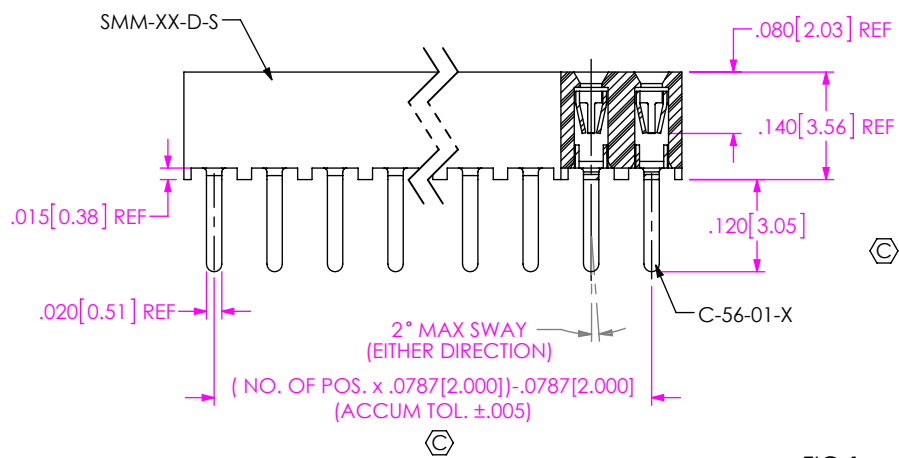
FIG 1 -01: THROUGH HOLE
