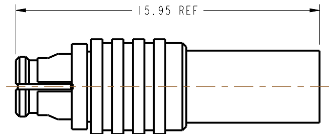
ASSEMBLED VIEW
