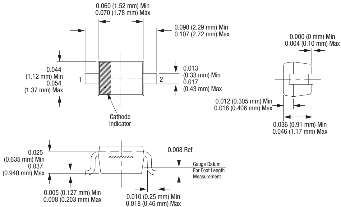
Figure 11. SOD-323 Package Dimension Drawing
