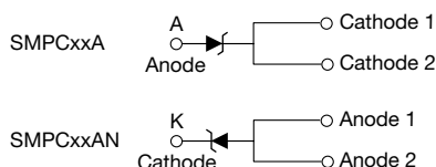
TO-277A (SMPC)
