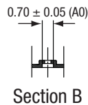
Figure 16. SOD-882 Tape and Reel Dimensions
