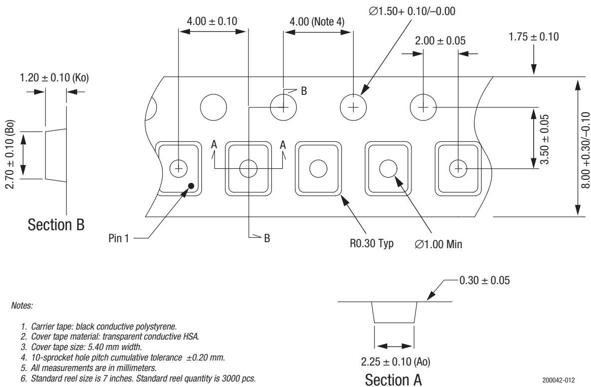
Figure 12. SC-88 Tape and Reel Dimensions
