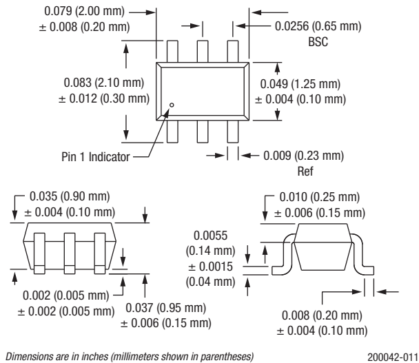
Figure 11. SC-88 Package Dimension Drawing
