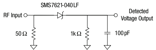
Broadband Detector Circuit
