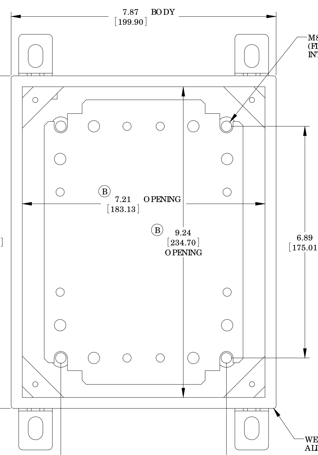
FRONT VIEW (LESS COVER)
