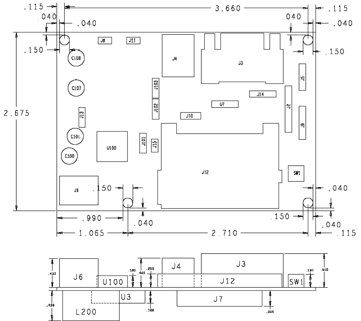
Figure A-1 Host Interface Board Dimensions
