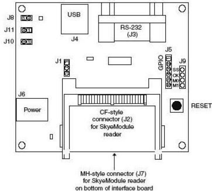
Figure B-1 Host Interface Board, Top View
