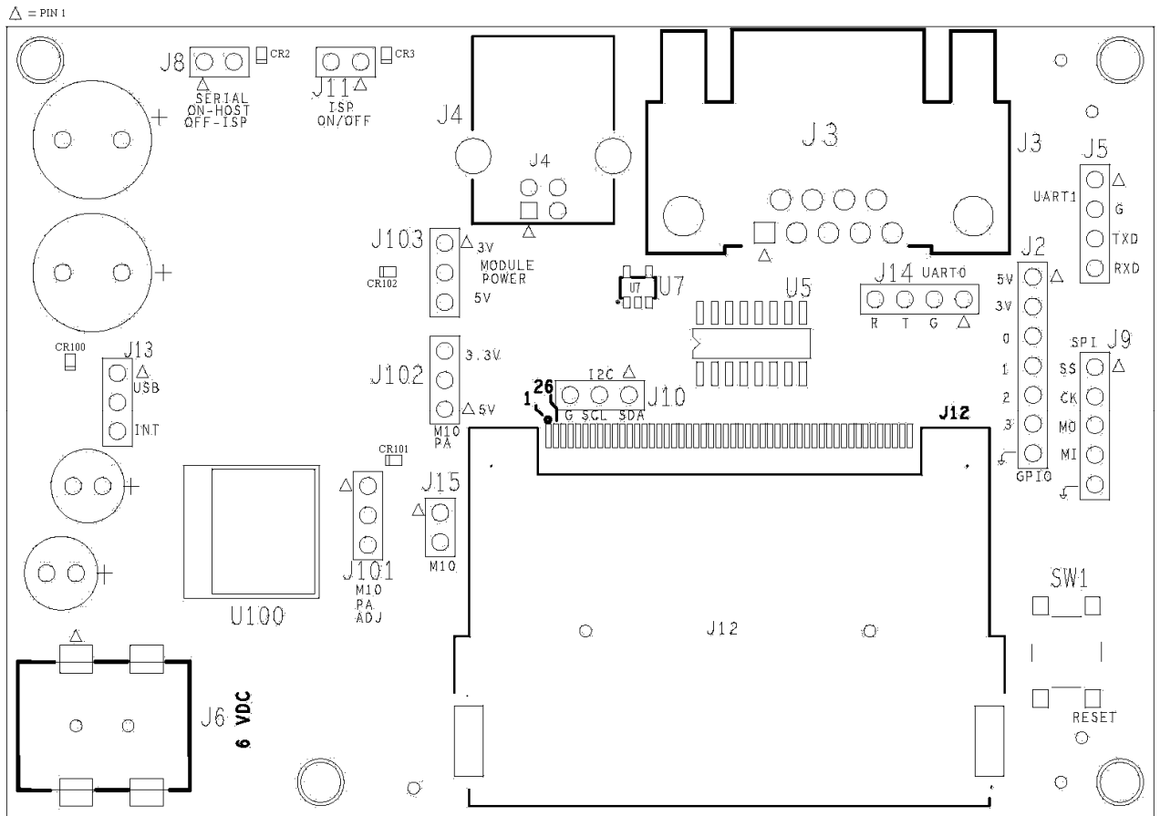
Figure A-2 shows a top view of the host interface board including connectors.
