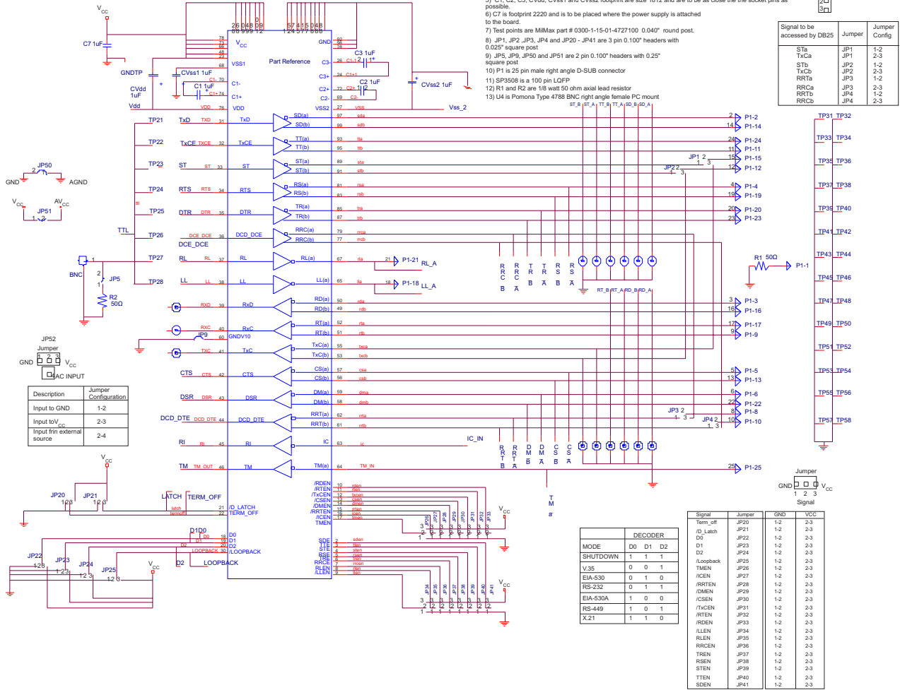
Figure 1. SP3508 Schematic
