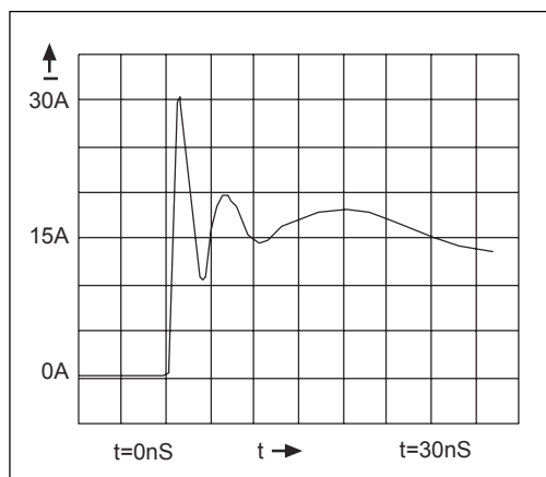
Figure 37. ESD Test Waveform for IEC1000-4-2
