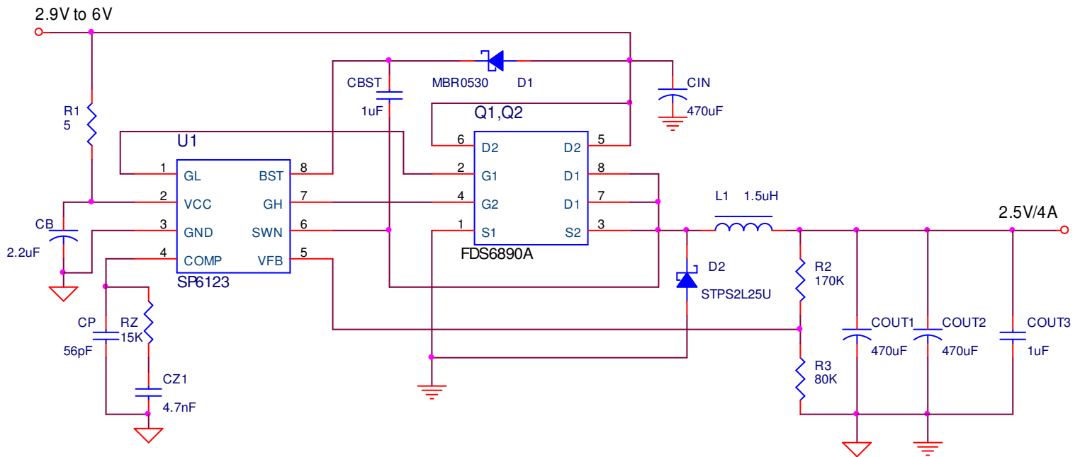
SP6123 Demo Board Schematic.
