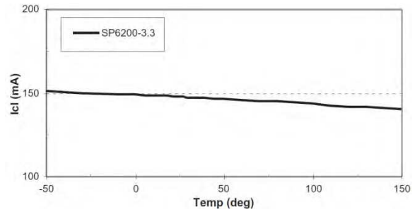
Fig. 21: Current Limit vs. Temp (fixed 3.3V, V_{IN} =4V)
