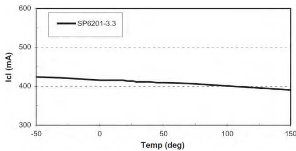
Fig. 20: Current Limit vs. Temp (fixed 3.3V, V_{IN} =4V)
