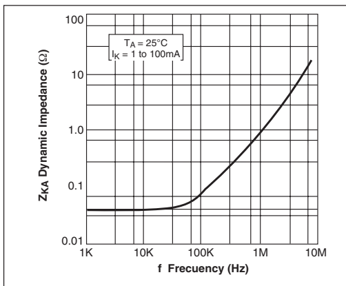
Figure 18. Dynamic Output Impedance T_A = 25^\circ\text{C} , I_k = 1 \text{ to } 100\text{mA}
