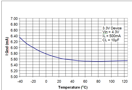
Fig. 12: Ground Current vs Temperature I_{LOAD} = 500\text{mA}
