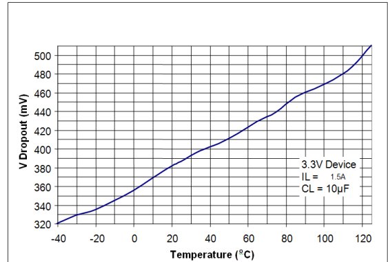
Fig. 17: Dropout Voltage vs Temperature I_{\text{LOAD}} = 1.5\text{A}
