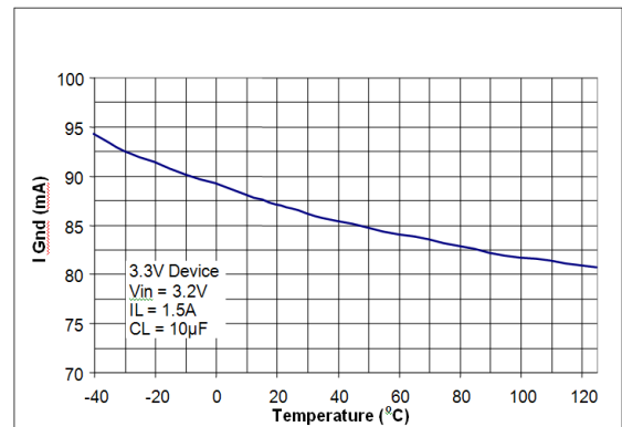
Fig. 15: Ground Current vs Temperature Dropout, I_{LOAD} = 1.5\text{A}
