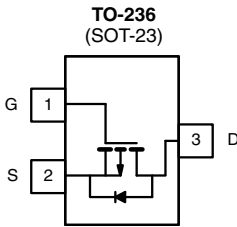
Top View SQ2309ES*
