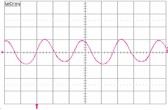
Figure 13. Input reflected ripple-current, i_c (100 mA/div.), measured at input terminals at full rated load current and V_{in} = 48 V. Refer to Fig. 12 for test setup. Time scale: 1 \mu s/div.
