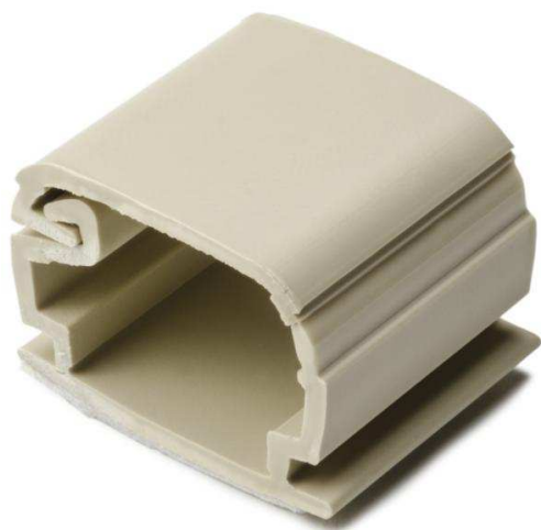
TSR Adhesive Cable Clamp, .76" Width, .51" Height, PVC, Ivory, 100/pkg
