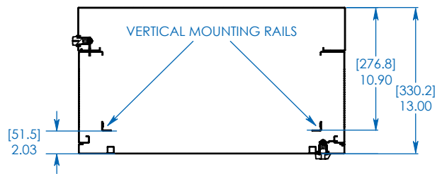
CROSS-SECTION A: CLEARANCE IN FRONT OF AND BEHIND VERTICAL MOUNTING RAILS (RAILS AT DEFAULT POSITION)
