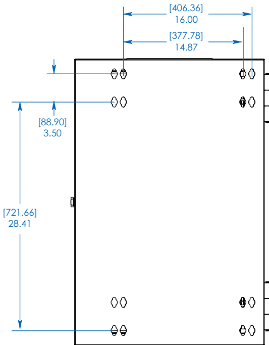
REAR VIEW
