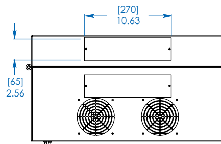
TOP/BOTTOM VIEW
