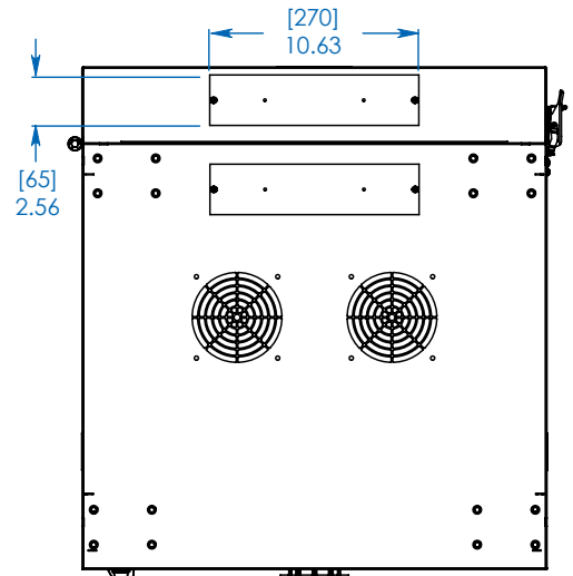
TOP/BOTTOM VIEW
