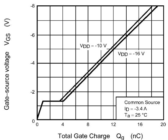
Fig. 7.12 Dynamic Input/Output Characteristics
