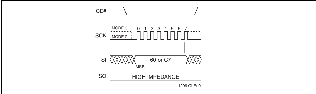
FIGURE 4-13: CHIP-ERASE SEQUENCE
