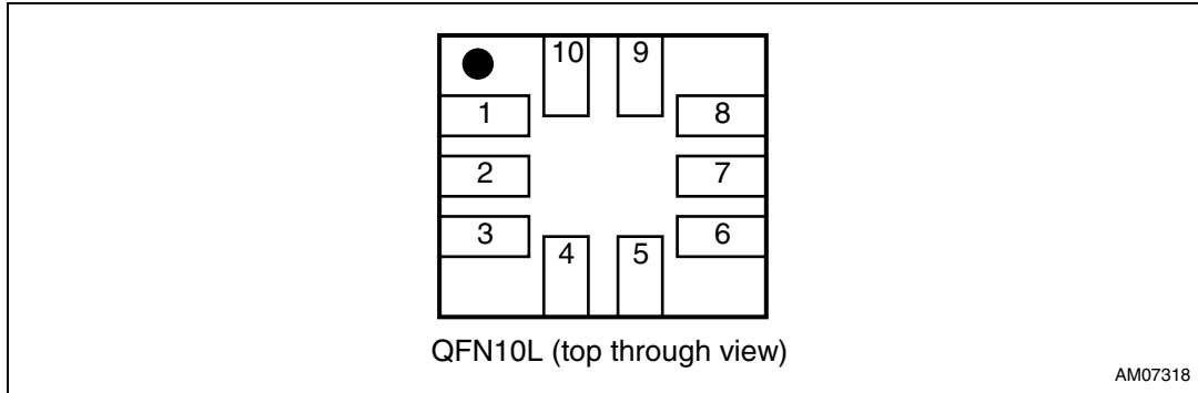
Figure 1. Pin configuration
