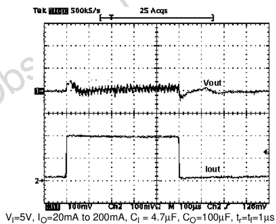
Figure 15 : Load Transient
