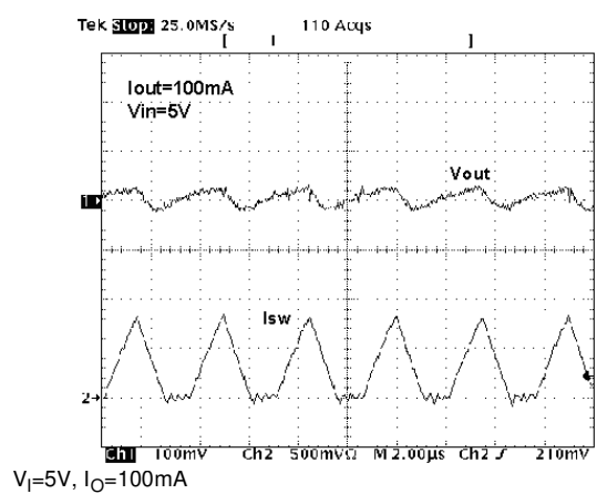
Figure 18 : Switching Waveform
