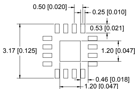
Recommended PCB Soldermask (SMOBC) for Land Pattern(dimensions in mm[in]):
