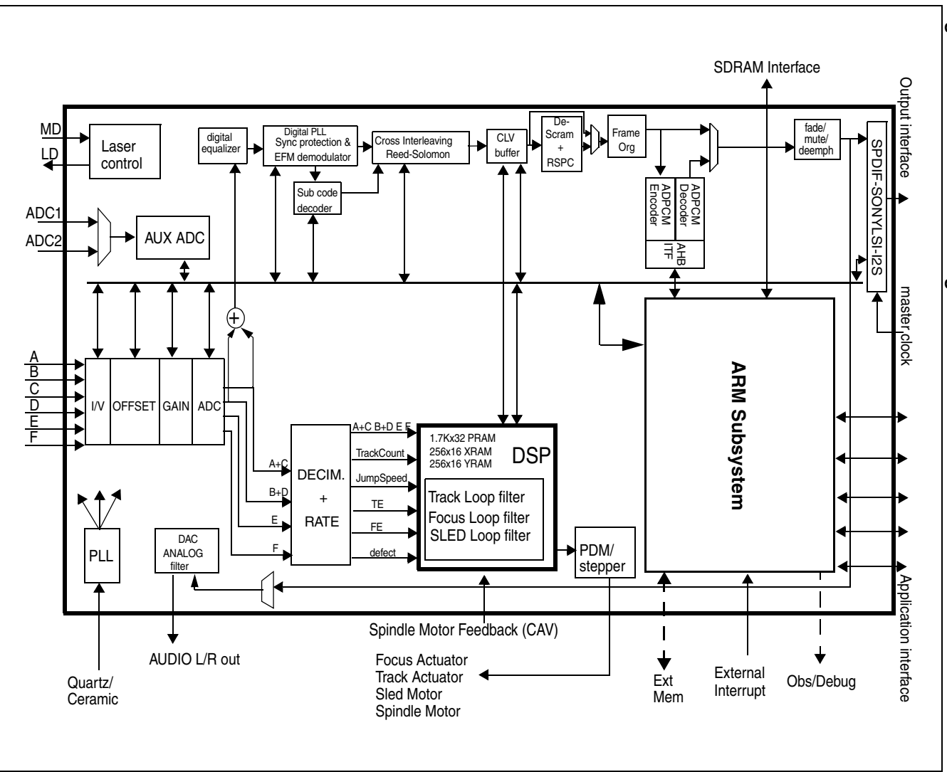
Figure 1. STA1052 block diagram
